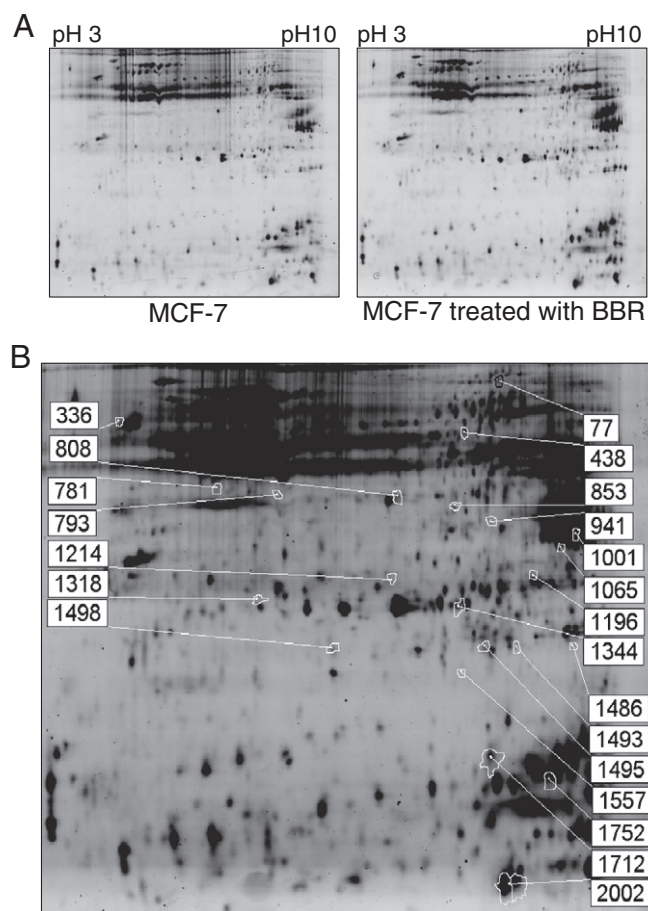
Fig. 6 – Redox 2D-DIGE analysis of berberine-induced differential cysteine-modification in MCF-7 cells. (A) Lysates from MCF-7 cells treated with 100 \mu\text{g}/\text{mL} of berberine or left untreated were subjected to redox 2D-DIGE analysis as described in Materials and methods . Images of protein samples from untreated and berberine-treated MCF-7 are displayed. (B) Differentially labeled protein features are annotated with spot numbers.
